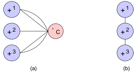
Figure 2: (a) RV-graph ( \rho + C ): there is an edge between a request and a vehicle for every feasible route plan in which a vehicle can service the new request. (b) VV-graph ( \rho + \rho ): an edge between vehicle E^8 and E^9 represents the swap with the highest utility between the two vehicles.
