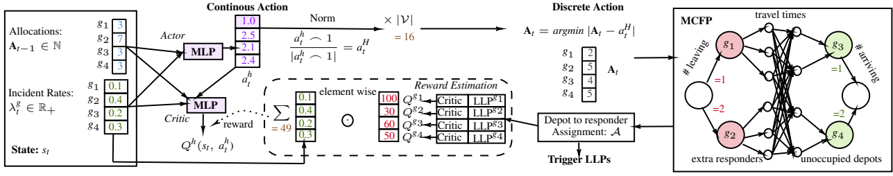
Figure 3: Overview of the training process of the high-level RL agent using DDPG. First, we map the state to a fixed-size feature vector and feed it into the MLP-based actor to generate the continuous action ( \mathbf{a}_t^h ). Next, we discretize the continuous action and feed it into the minimum-cost flow problem to generate the assignment of responders to depots ( \mathcal{A} ). After that, we trigger those LLPs whose regions were affected by the high-level reallocation. Finally, we use the critic to judge the performance of the actor by training the critic with rewards estimated by the LLP critics.
