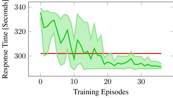
Figure 7: Evolution of the performance of the policy \mu_h throughout the training process for the high-level decision agent of the 7-region decomposition in Nashville , measured as the average response time. The dark green line (■) indicates the average of 5 different policies (trained on the given number of episodes), which are evaluated on 5 different sample chains with the number of responders in the entire city ranging from 24 to 28. The light green area (■) indicates the 10th to 90th percentiles of average response times over 5 different policies. The red line (■) indicates the average response times obtained when using the state-of-the-art MCTS approach on the same 5 sample chains with the number of responders in the entire city ranging from 24 to 28.
